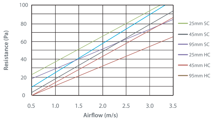
Filtro Pleat - Airflow vs. Initial Resistance
